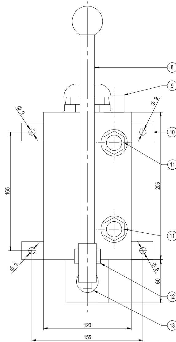
FRONT VIEW
